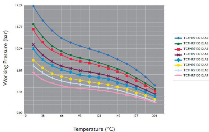
Furon HP PFA Pipe - Working Pressures
