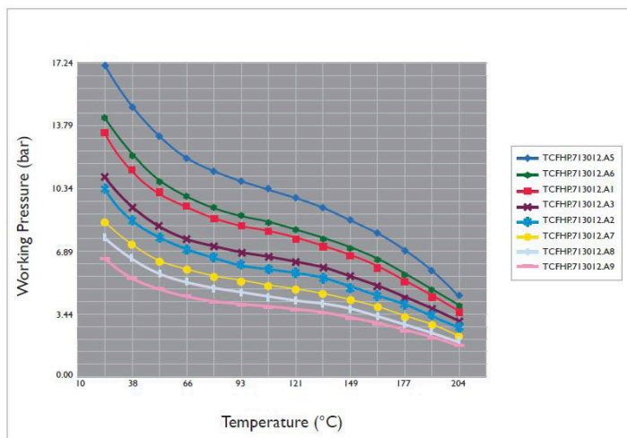
Furon HP PFA Pipe - Working Pressures
