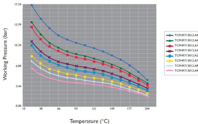
Furon HP PFA Pipe - Working Pressures
