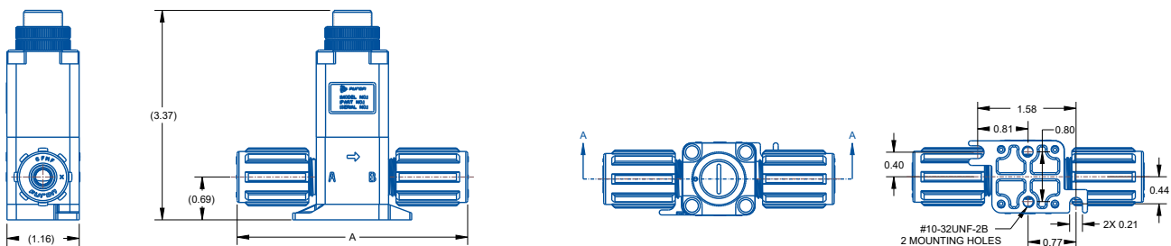
Saint-Gobain's pressure relief valve solution is designed to limit upstream pressure to protect sensitive equipment. Settings are customizable and can be locked into a tamper-proof position.
